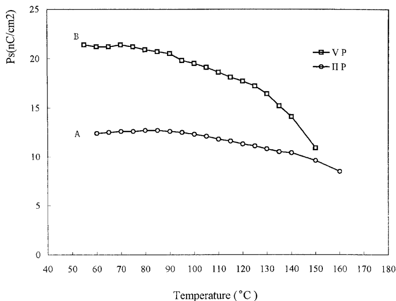
Figure 8. Spontaneous polarization P_s versus temperature for polymer IIP (○) and VP (■).
